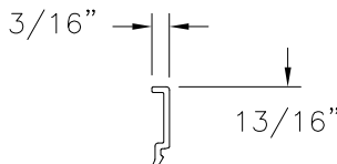
GLAZING BEAD (DT1770-R) EXTRUDED RIGID PVC
