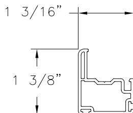
SASH STILE (CH9008) EXTRUDED RIGID PVC
