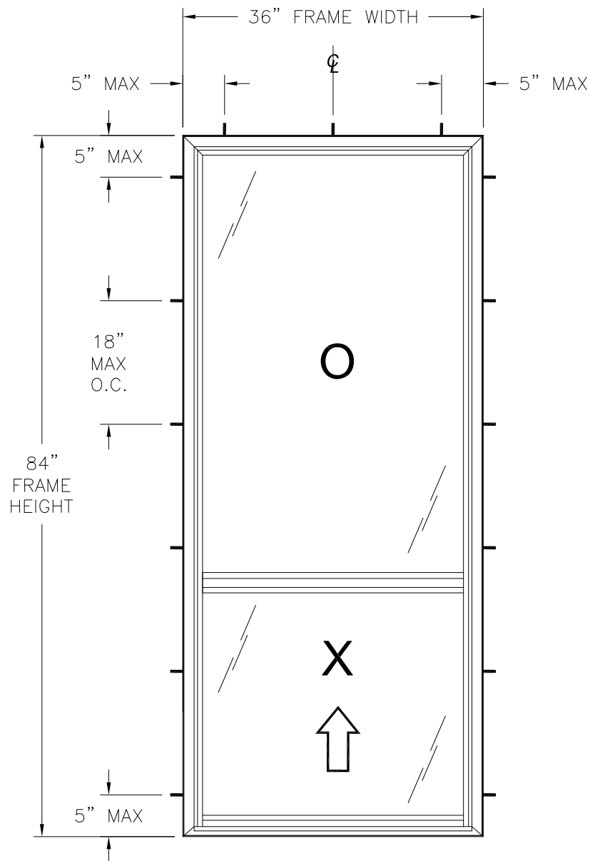
220 VINYL SINGLE HUNG WINDOW EXTERIOR VIEW
